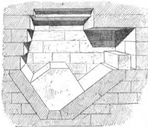
FIG. 151.—Portcullis closed.
